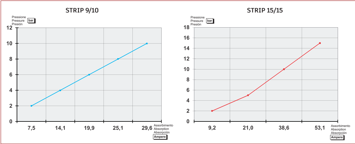
Curve rendimenti - Performance curves - Curvas de rendimiento
