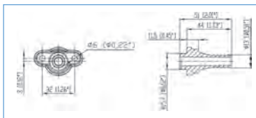
Kit lato pompa - Pump side kit - Kit lado bomba
