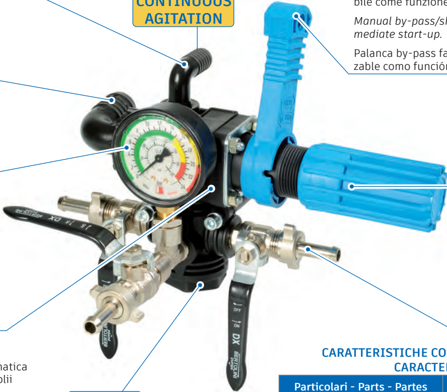
ANTIDRIP SYSTEM
